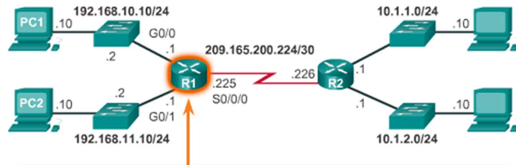
Configure the Loopback0 Interface
